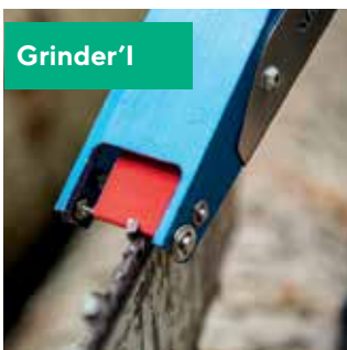
Sharpening Grinder
